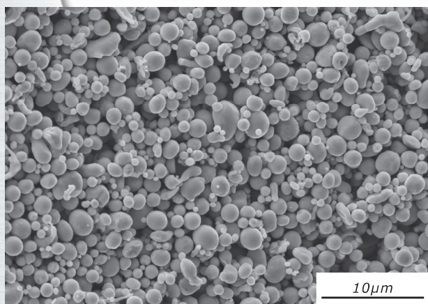
Cu-HWQ 1.5 \mu\text{m} (SEM image \times 100 )
